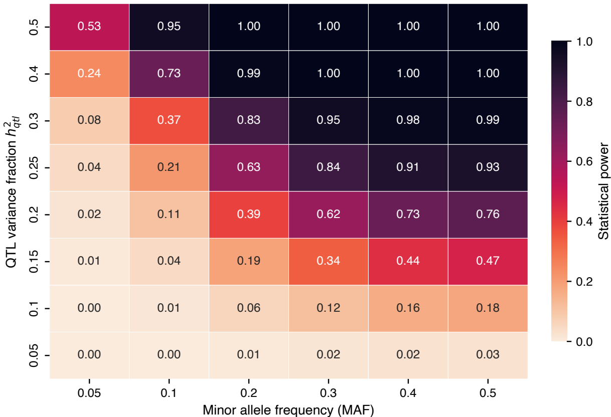
GWAS power — n = 105, Bonferroni \alpha = 2.99\text{e-}05
