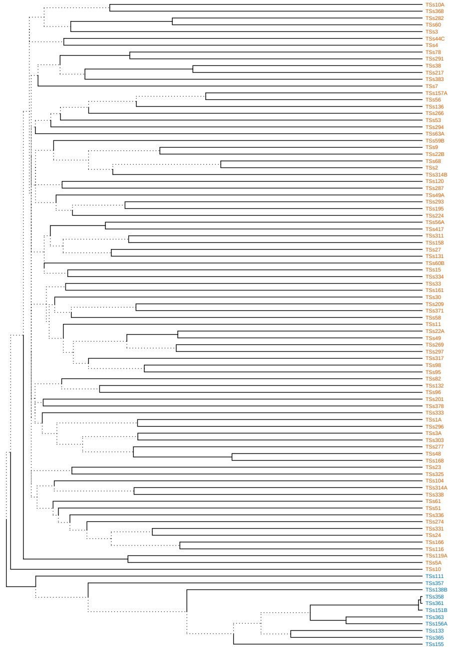
IQ-TREE
