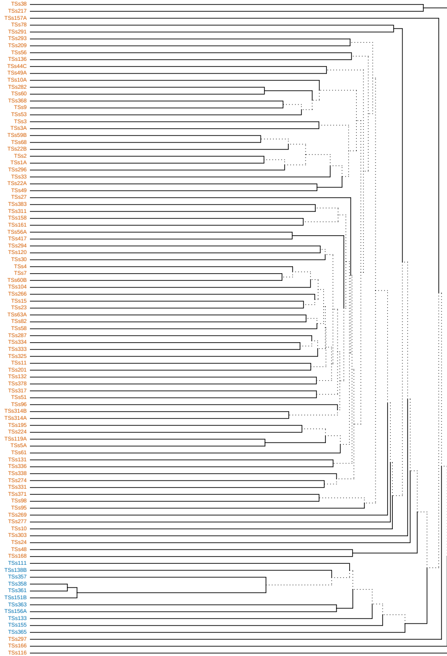
UPGMA
