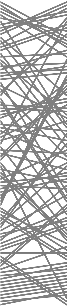
IQ-TREE vs UPGMA (entanglement = 0.152)
