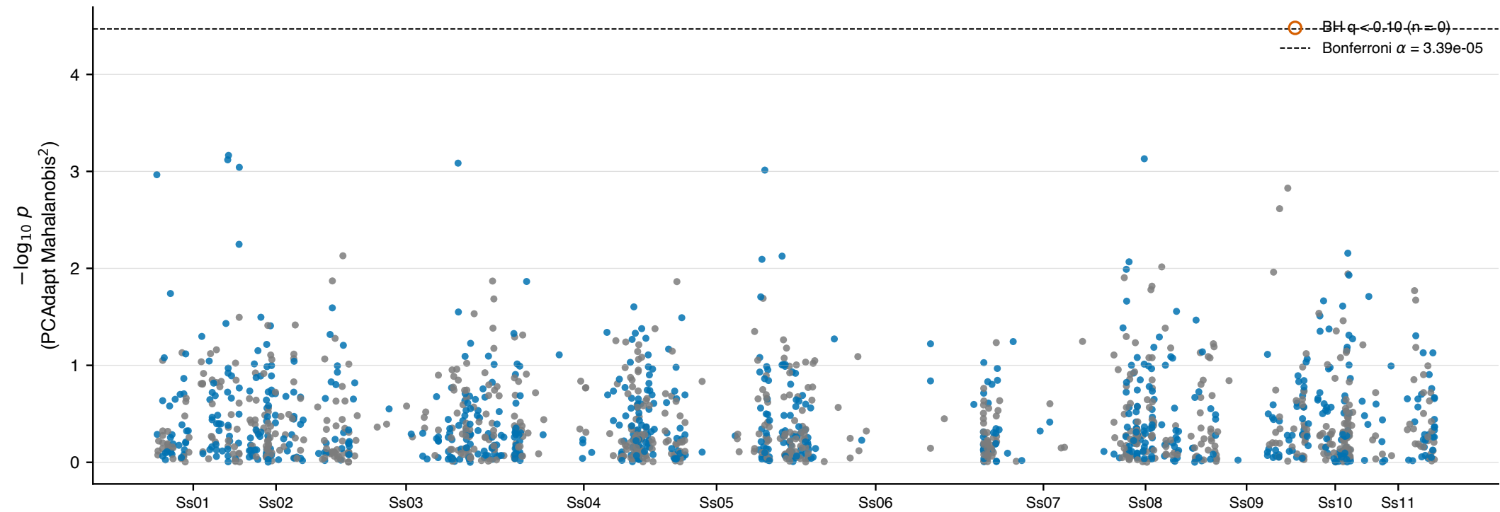
PCAdapt-style F_{ST} outlier scan, K = 2 PCs
