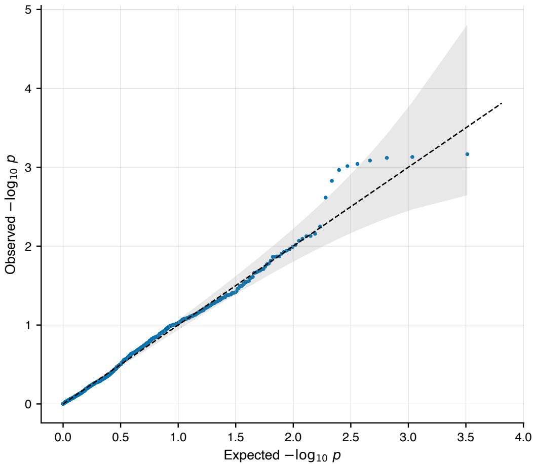
PCAdapt QQ — n = 1625 markers; \lambda_{GC} = 0.93
