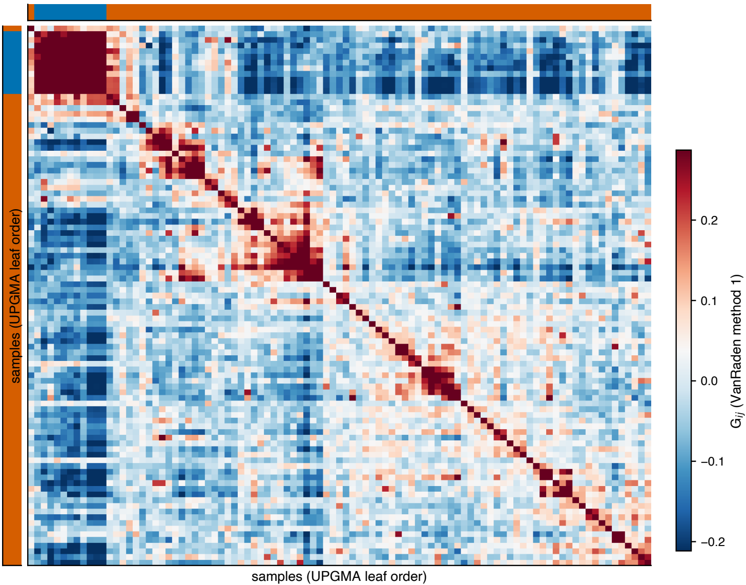
Genomic relationship matrix — reordered by UPGMA on (1 - G)
