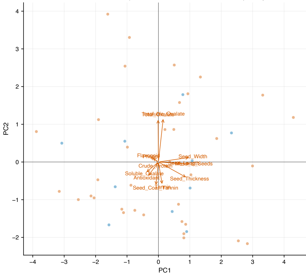
Trait PCA, all 13 traits (n = 45; PC1 + PC2 = 43% variance) — biplot
