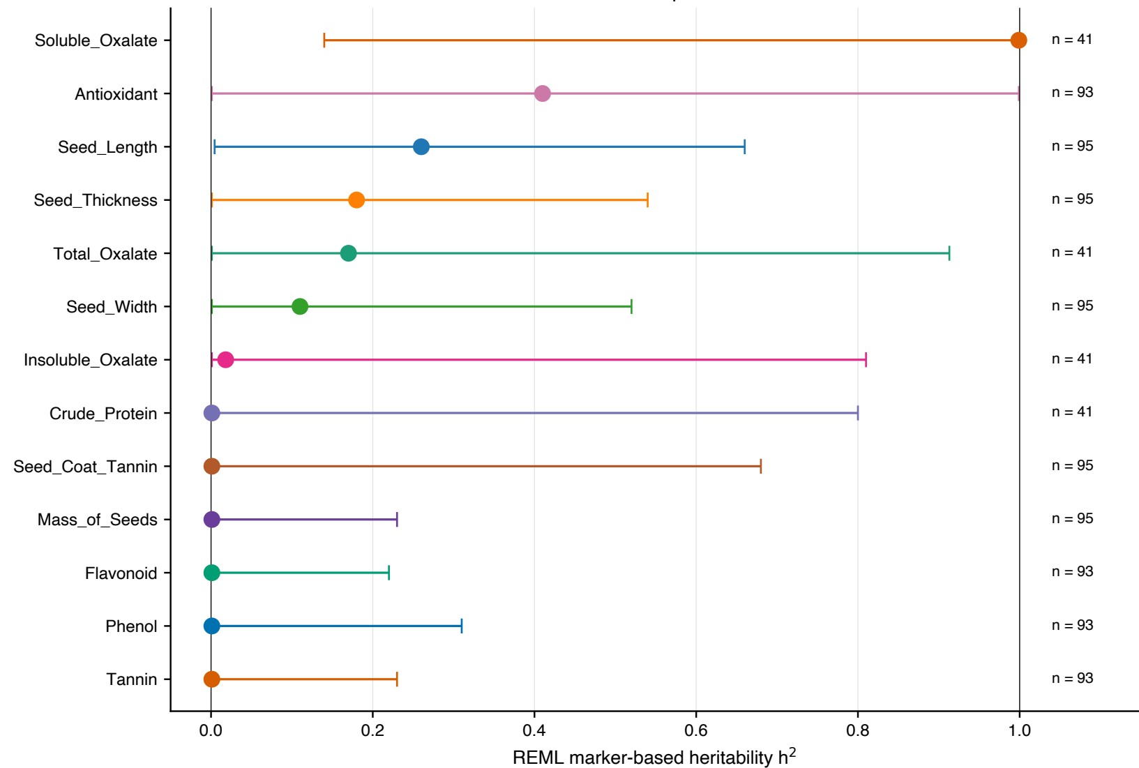
REML h^2 MLE + 95 % profile-likelihood CI
