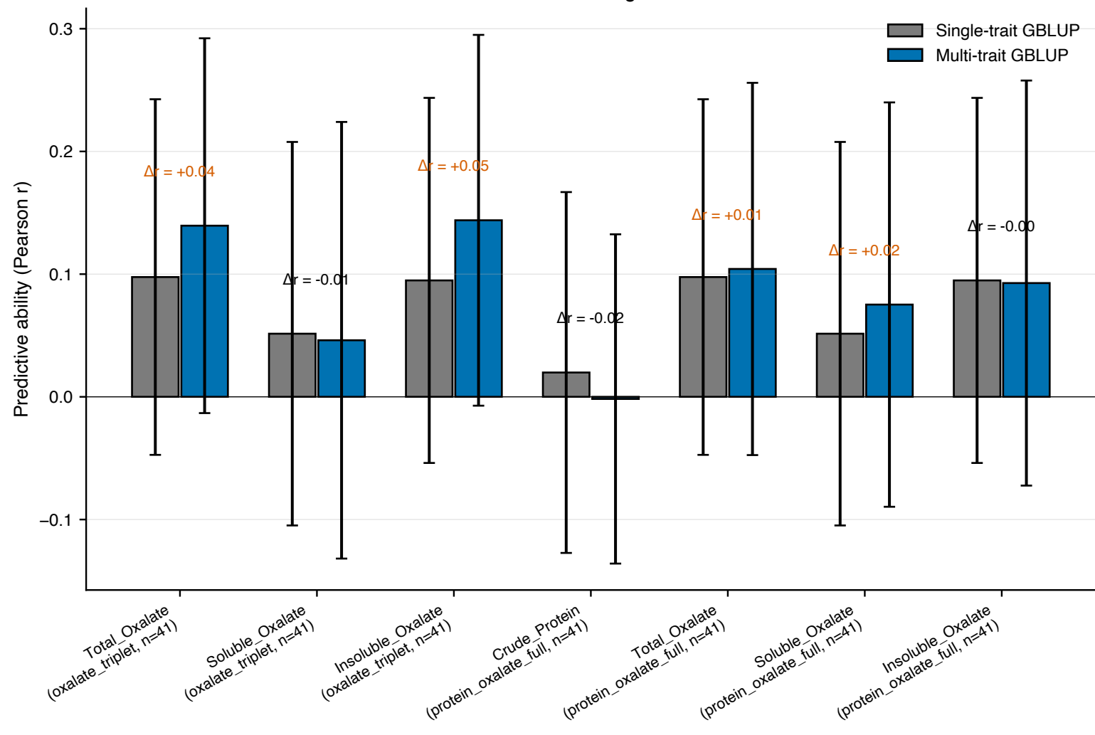
Multi-trait GBLUP vs single-trait baseline
