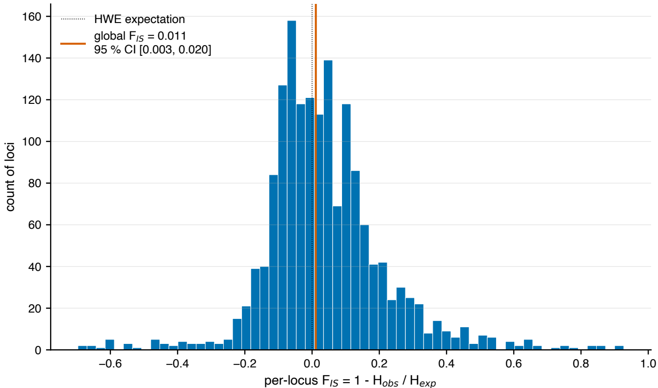
Per-locus F_{IS} across 1,625 AYB loci (selfing-rate signature)
