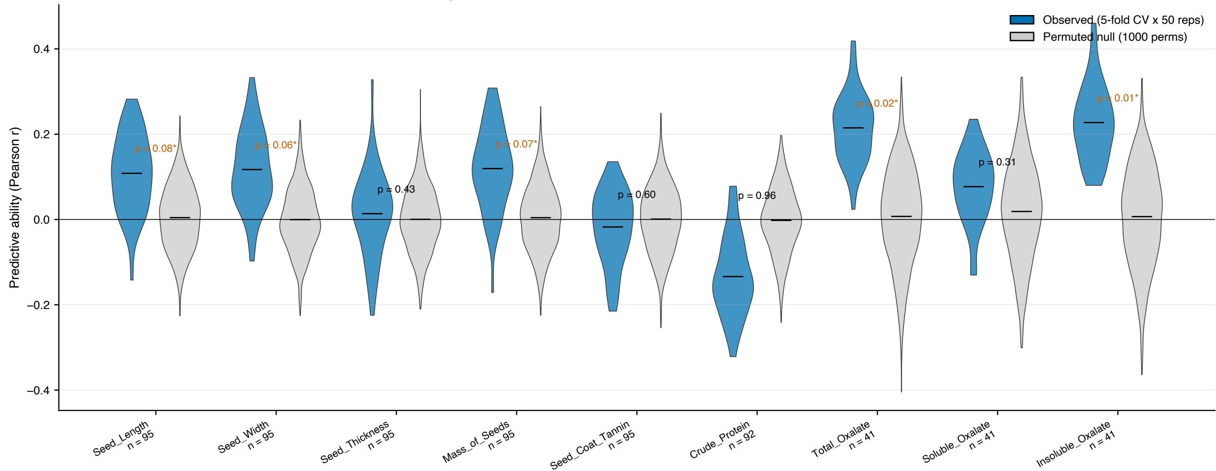
GBLUP genomic prediction across the 9 new AYB traits (per-rep distribution)
