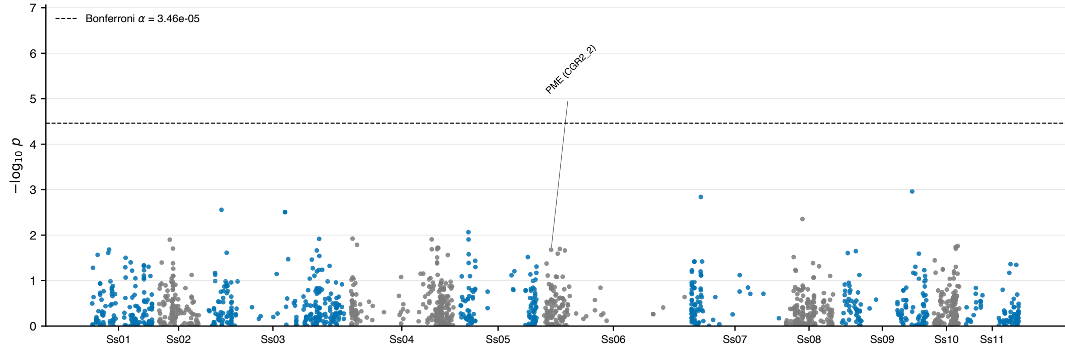
Mass_of_Seeds AYB-anchored (1,445 SNPs); top 30 scanned +/- 50 kb
