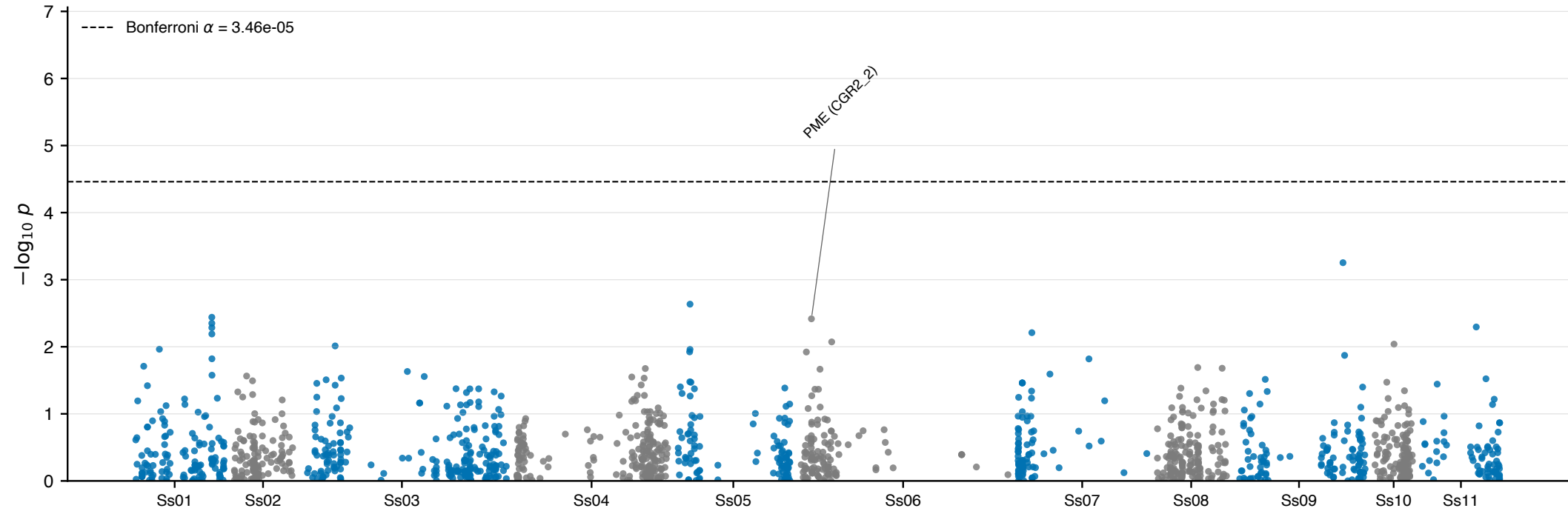
Seed_Length AYB-anchored (1,445 SNPs); top 30 scanned +/- 50 kb
