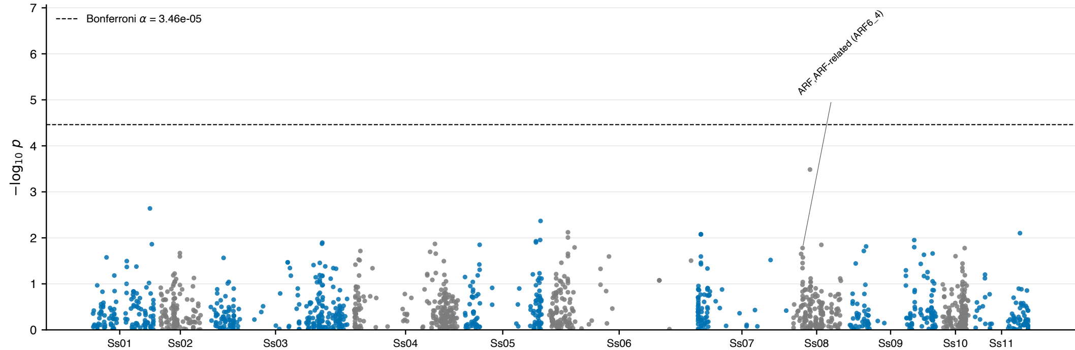
Seed_Thickness AYB-anchored (1,445 SNPs); top 30 scanned +/- 50 kb
