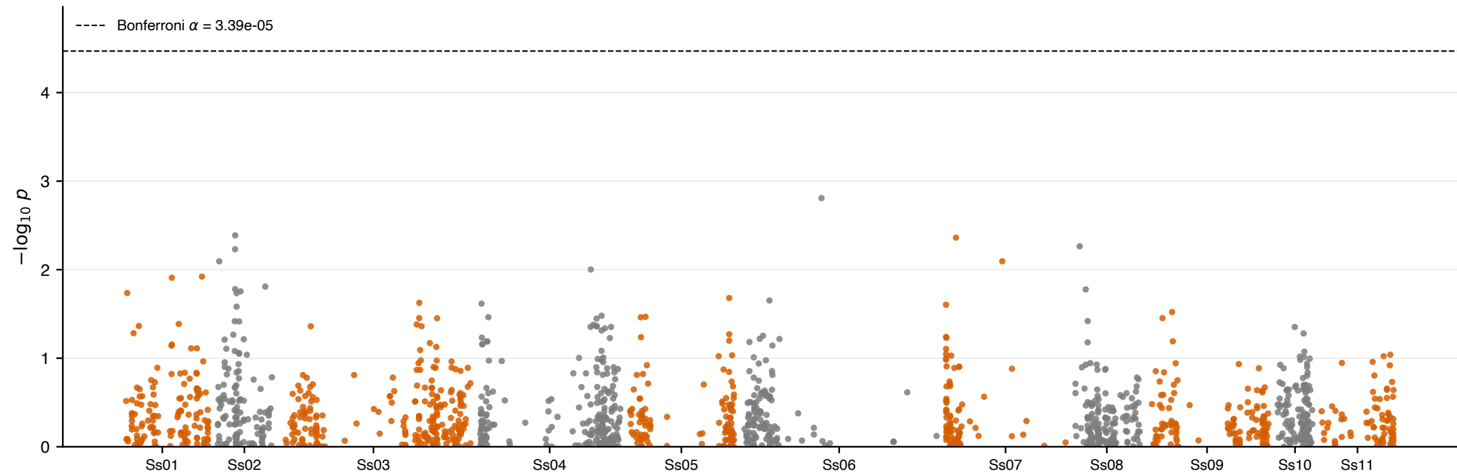
Tannin AYB-anchored (1,473 SNPs); top 30 scanned +/- 50 kb
