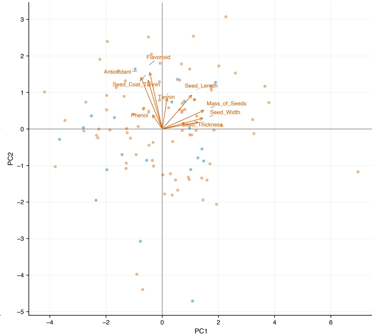
Trait PCA, 9 traits (n = 103; PC1 + PC2 = 57% variance) -- biplot
