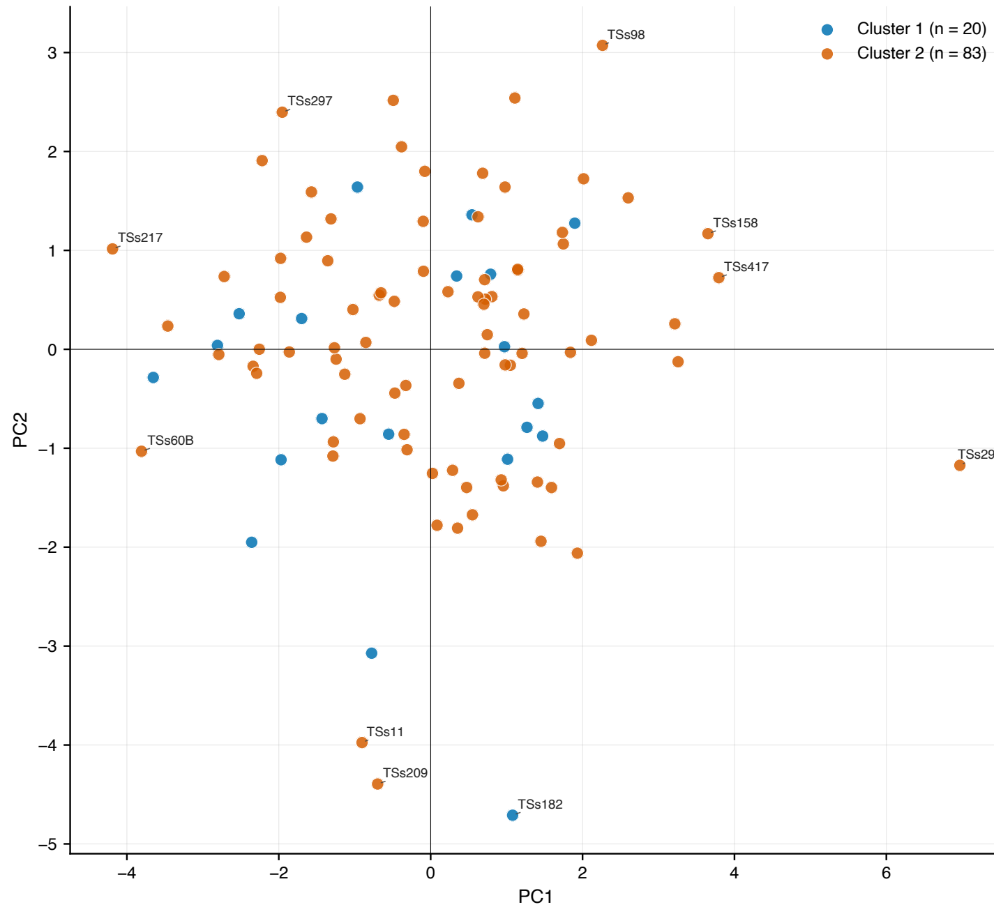
PCA scores -- coloured by marker-PCA cluster
