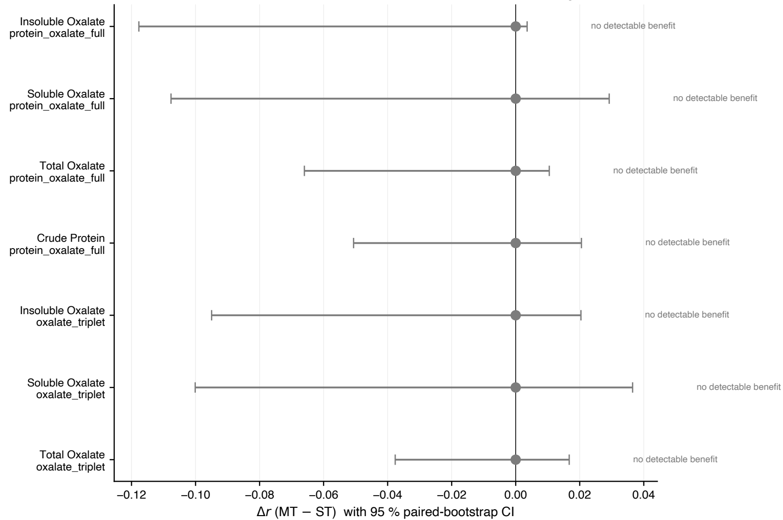
(B) Paired-bootstrap CI on the MT minus ST predictive-ability gain
