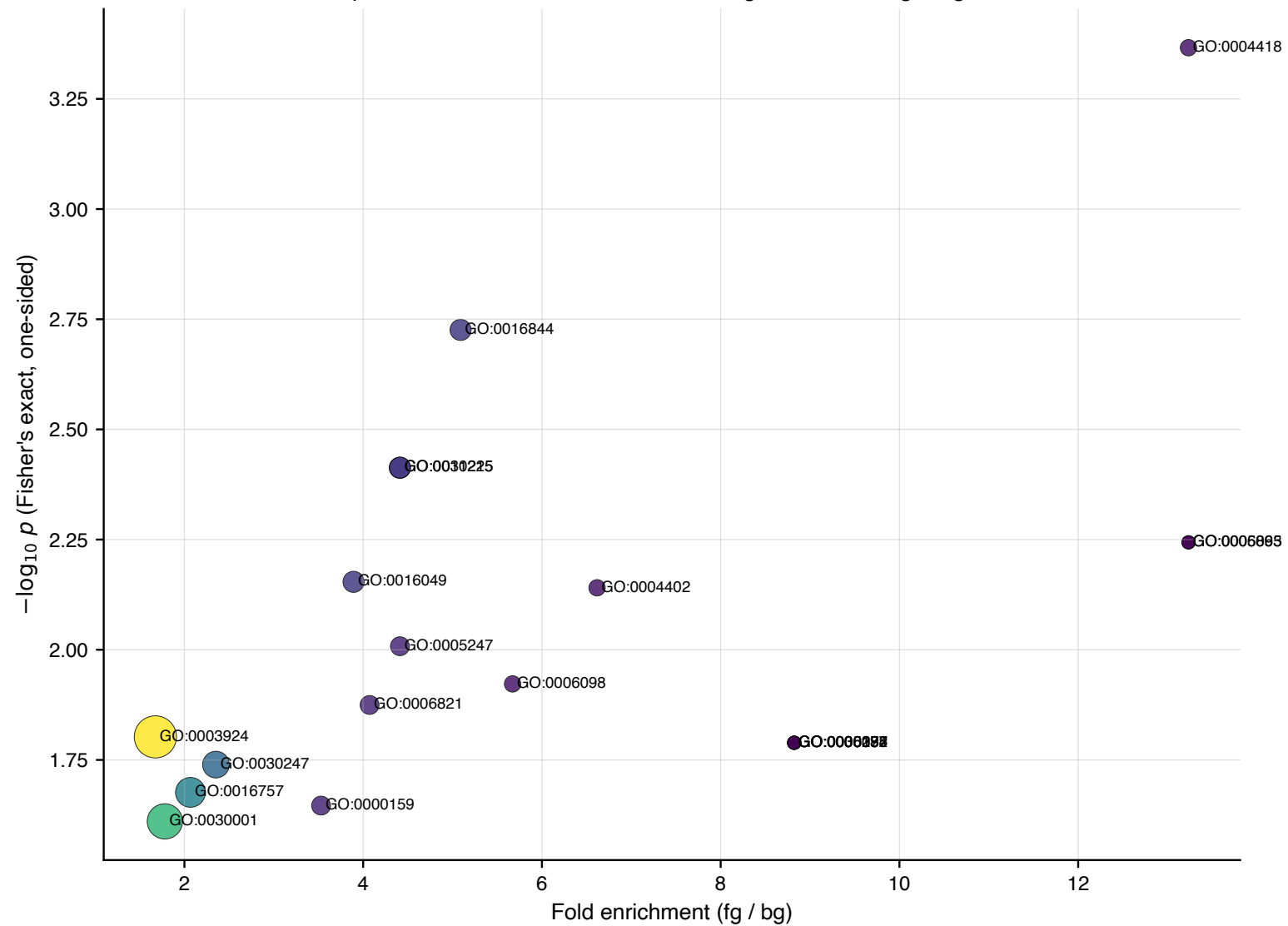
Top-20 most-enriched GO terms among candidate-region genes
