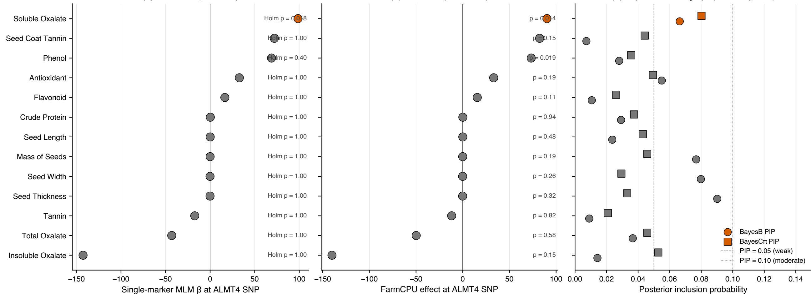
(A) MLM Wald (reference)
