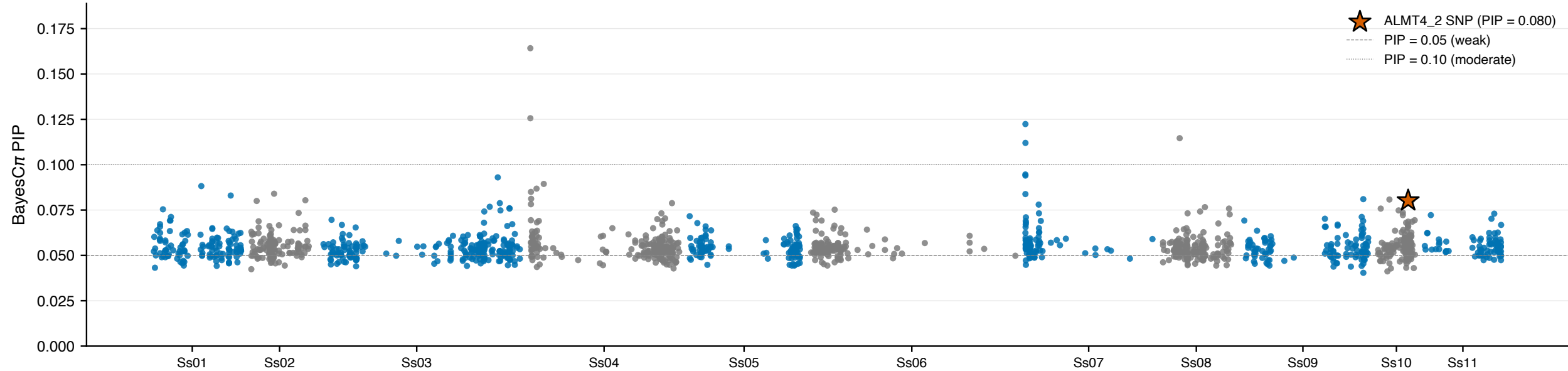
(B) BayesC \pi posterior inclusion probability per SNP — Soluble Oxalate
