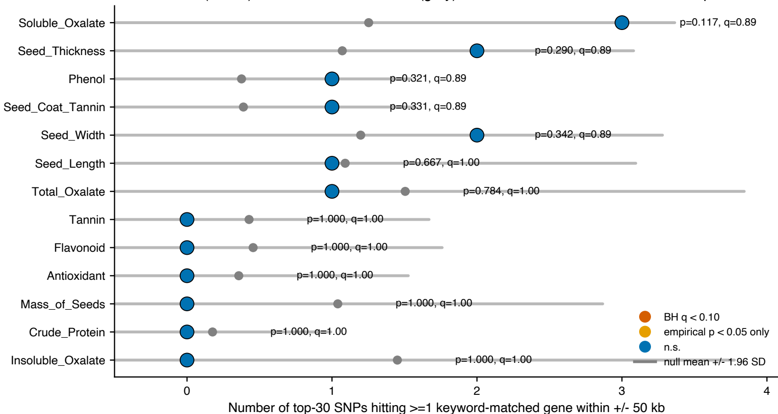
Permutation null on candidate-gene callout enrichment observed (colour) vs null mean \pm 1.96 SD (grey) across 1000 chromosome-stratified replicates
