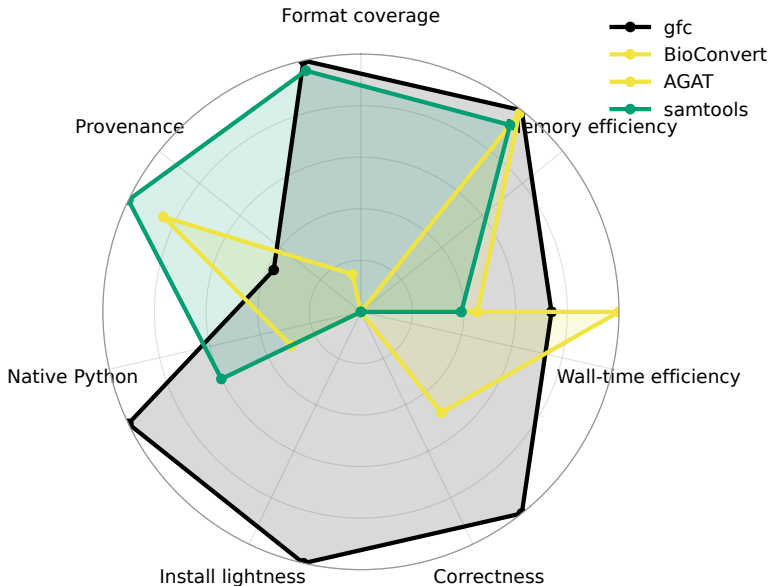
Capability spider — gfc vs three architecture classes
