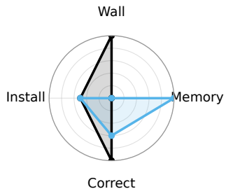
T6 — gfc vs pyhmmer
