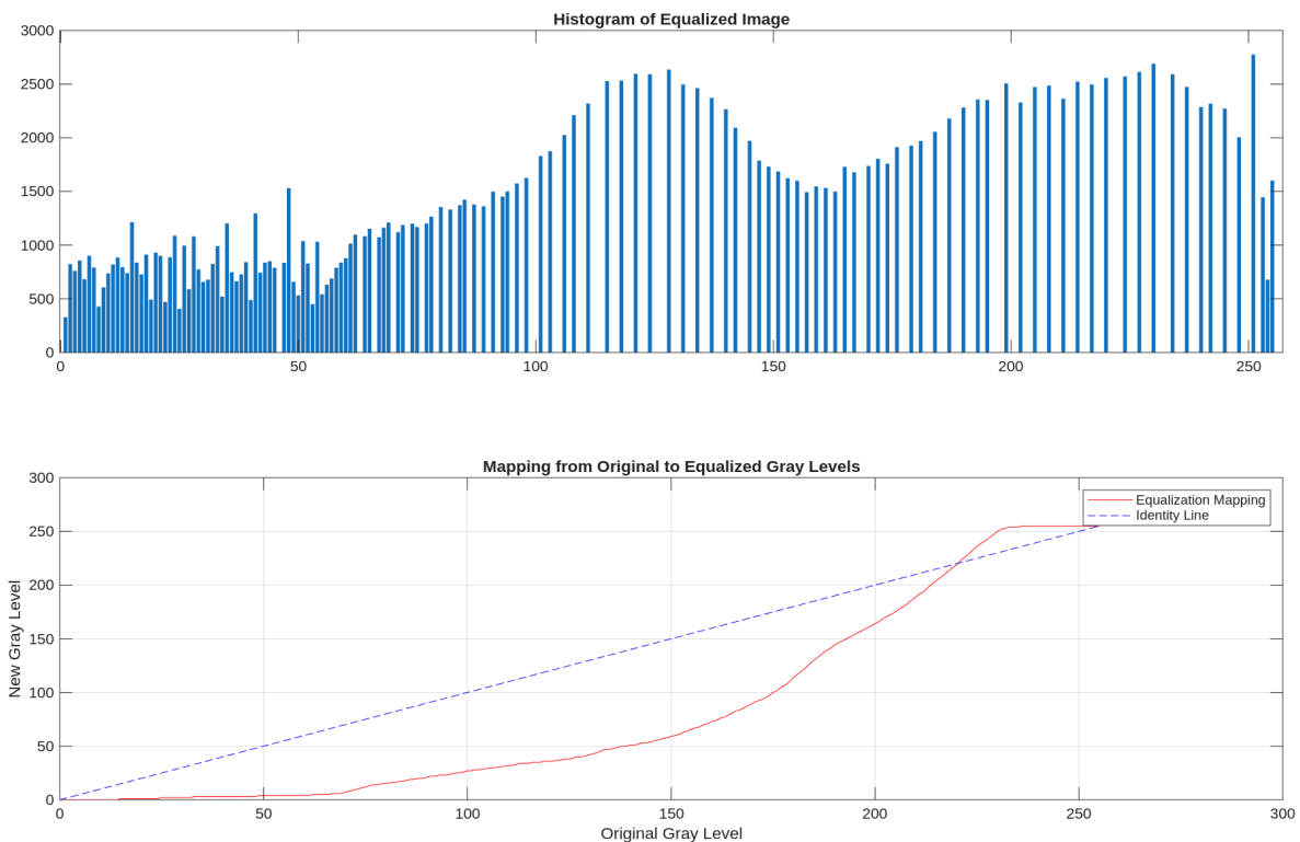
Figure 9: Histogram of equalized image and it's mapping
