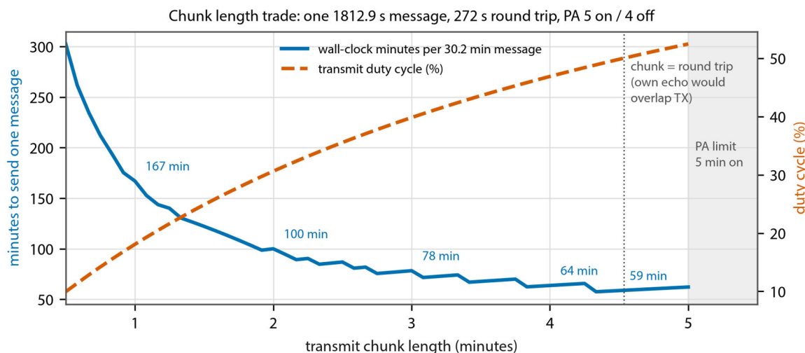
Figure 5 — Wall-clock time to send one 30.2-minute message and transmit duty cycle as a function of chunk length, for a 272 s round trip and the 5-on/4-off amplifier limit.
