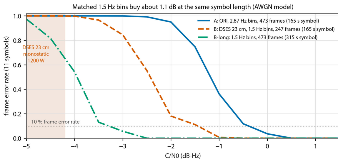
Figure 2 — Frame error rate versus C/N0 for ORI's Variant A and the DSES 23 cm Variant B, AWGN chi-square model with 4096 tones and 11 symbols. The shaded band is the DSES 23 cm monostatic link at 1200 W, from the date-resolved to the static albedo ( -5.4 to -4.2 dB-Hz).
