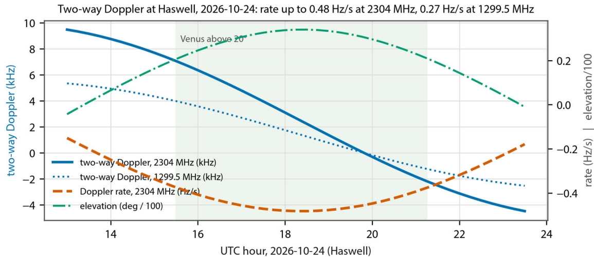
Figure 1 — Two-way Doppler shift at 2304 and 1299.5 MHz, Doppler rate at 2304 MHz, and Venus elevation at Haswell on 24 October 2026.
