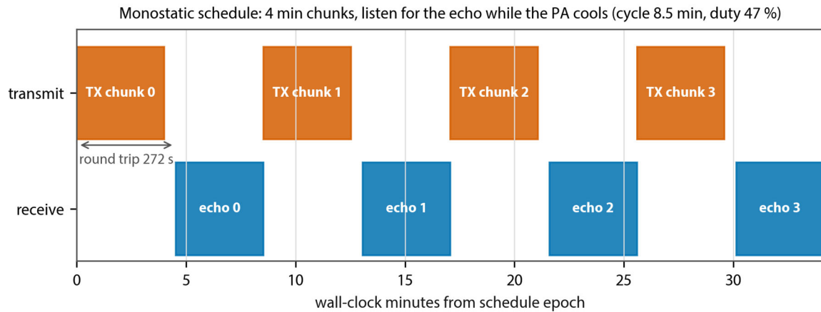
Figure 4 — Monostatic schedule with 4-minute chunks. Each chunk's echo returns 272 s after it was sent and is received while the amplifier cools; the next chunk follows the echo.
