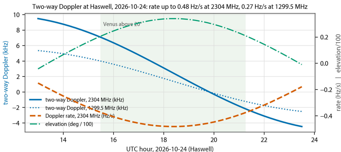
Figure 1 — Two-way Doppler shift at 2304 and 1299.5 MHz, Doppler rate at 2304 MHz, and Venus elevation at Haswell on 24 October 2026.
