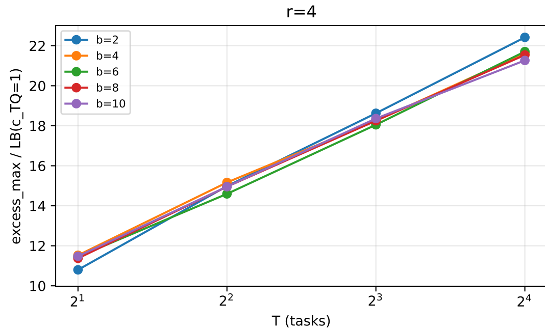
E4: achievability ratio vs T (flat = linear-T factor is analysis artifact)
