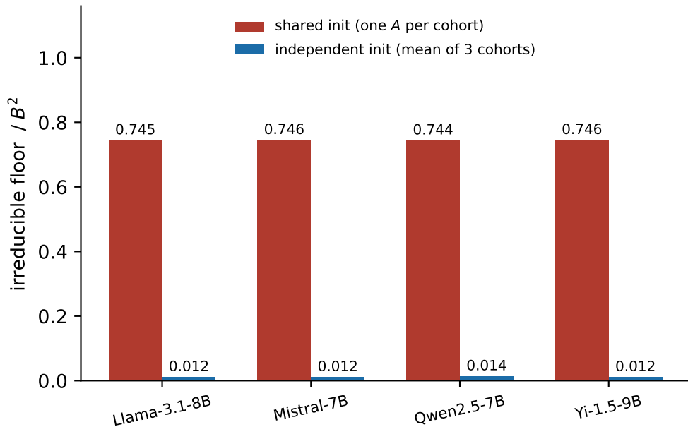
Lemma 2 floor B^2(1 - d_{\text{eff}}/(Tr)) moves by a factor of about 60
