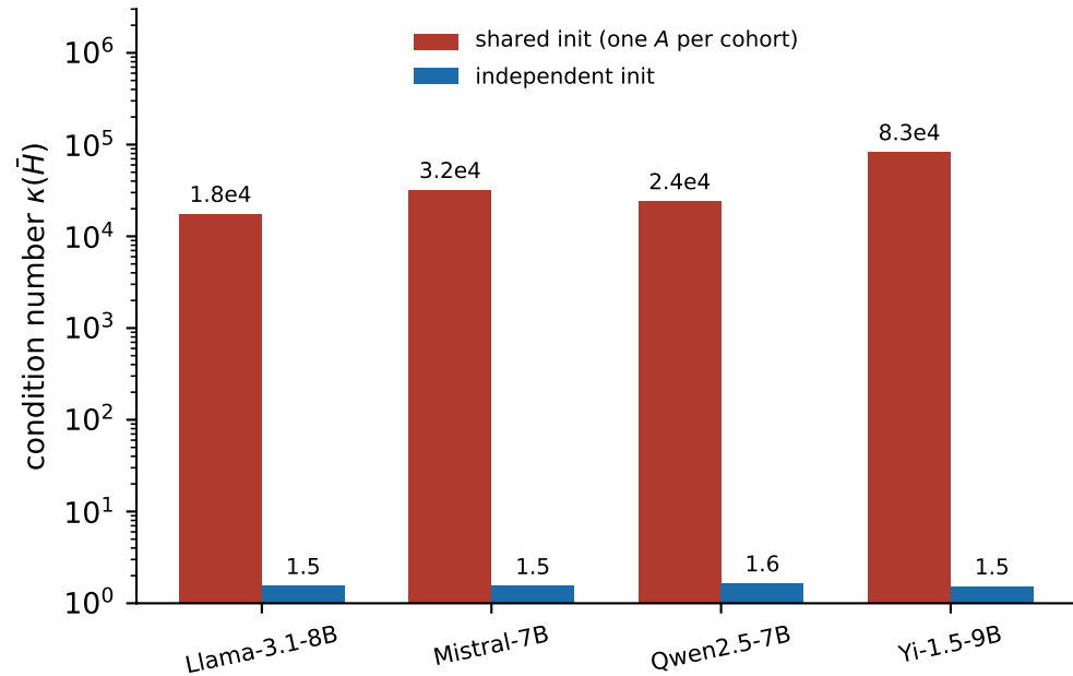
Conditioning, not the floor, is what initialisation controls
