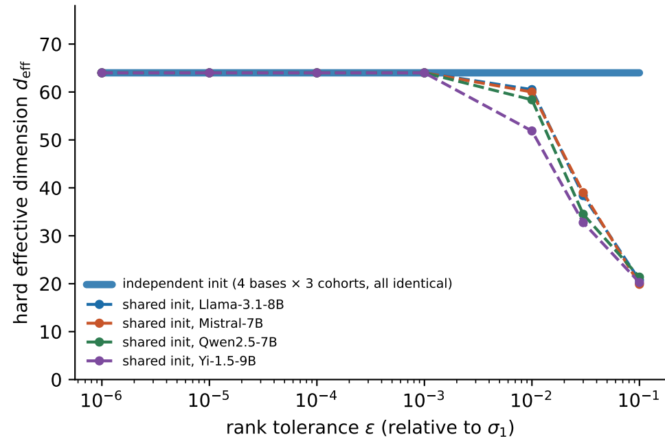
Effective dimension is tolerance-fragile only under shared initialisation
