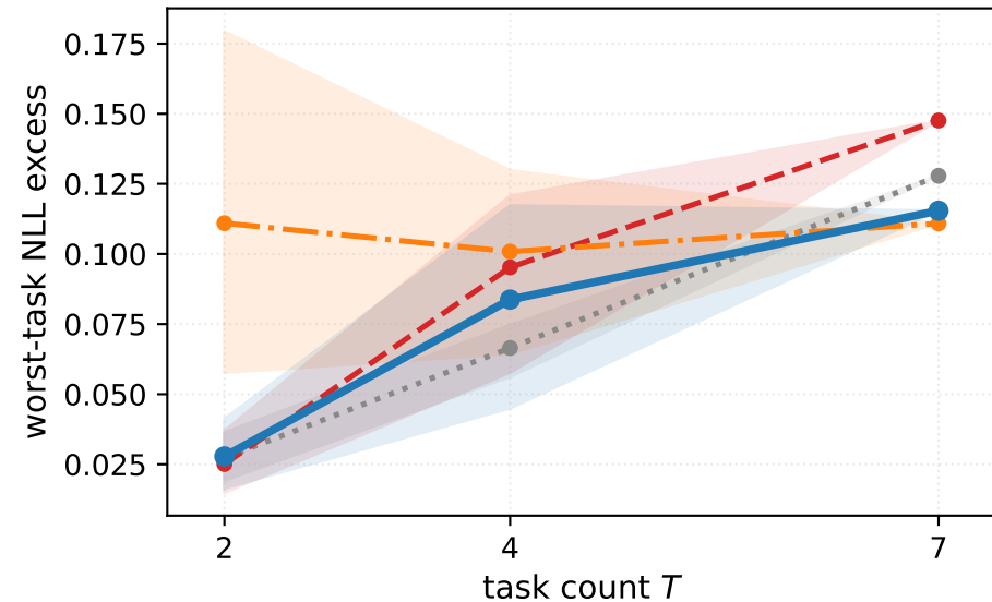
Yi-1.5-9B-Chat (saturated base)
