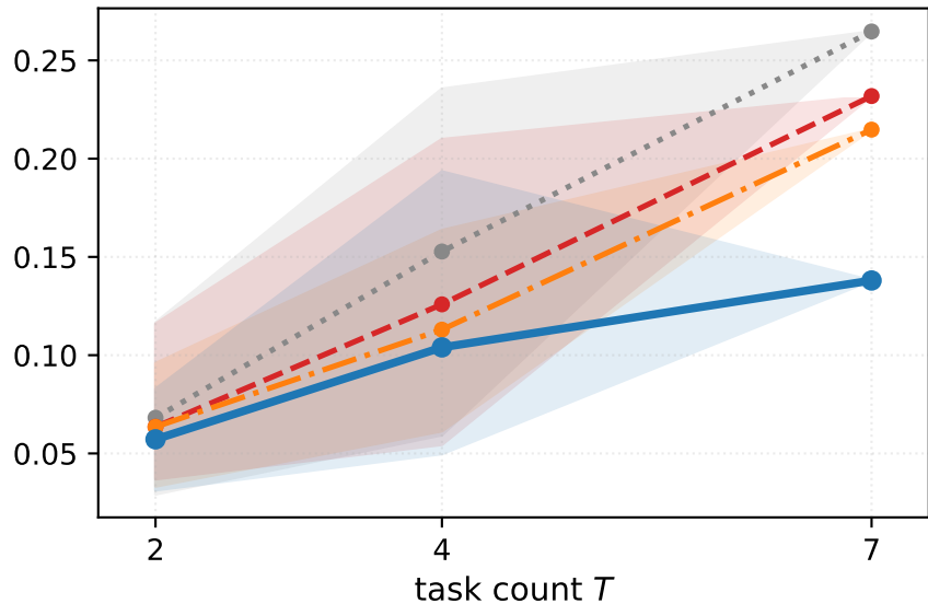
Llama-3.1-8B-Instruct (non-saturated)
