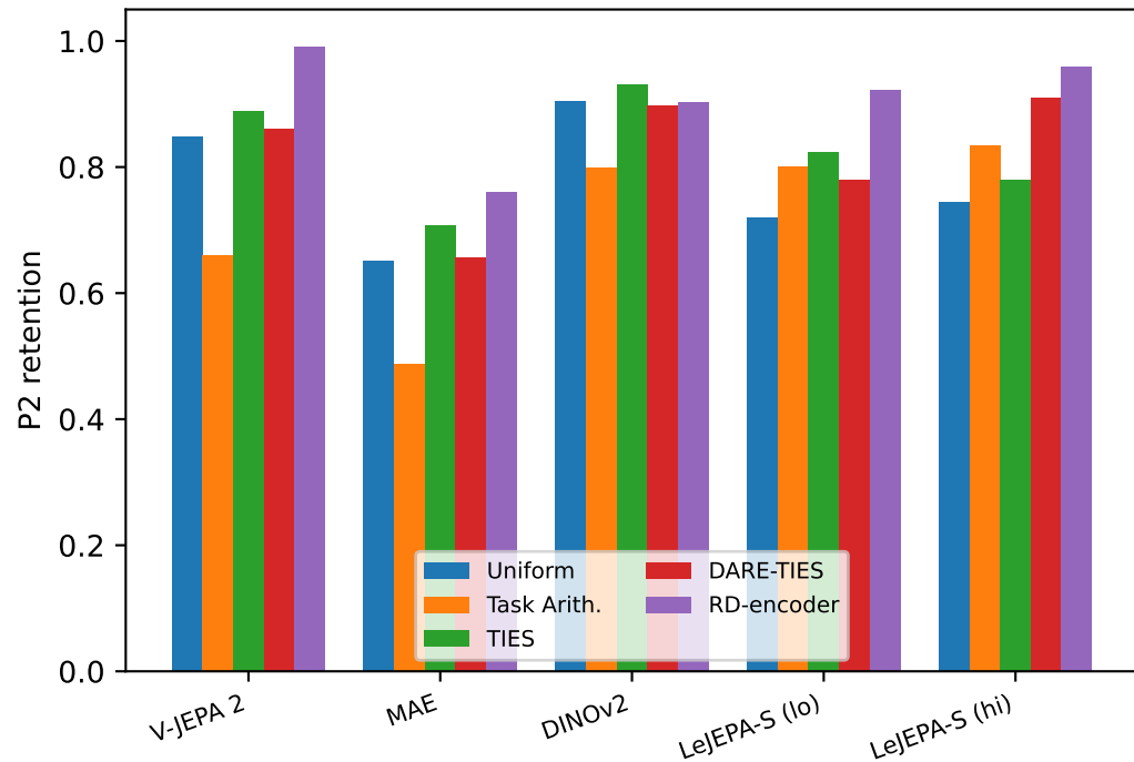
(b) RD-encoder best on 4/5 backbones
