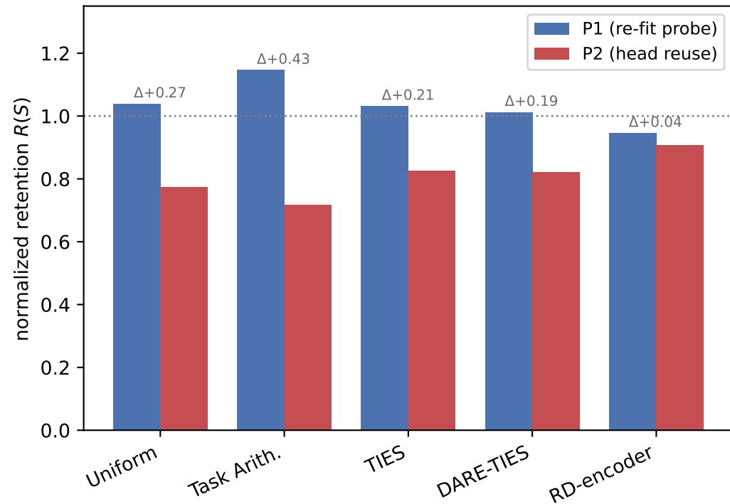
(a) Interference lives in the head (pooled)
