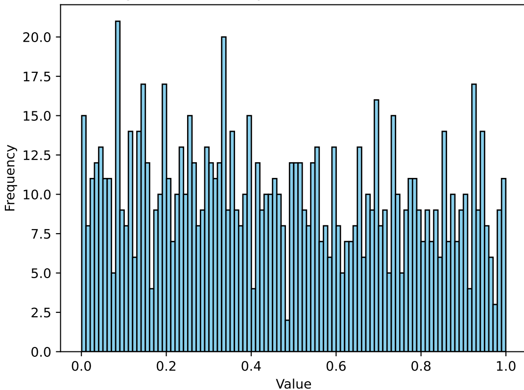
Histogram of Uniformly Distributed Random Numbers
