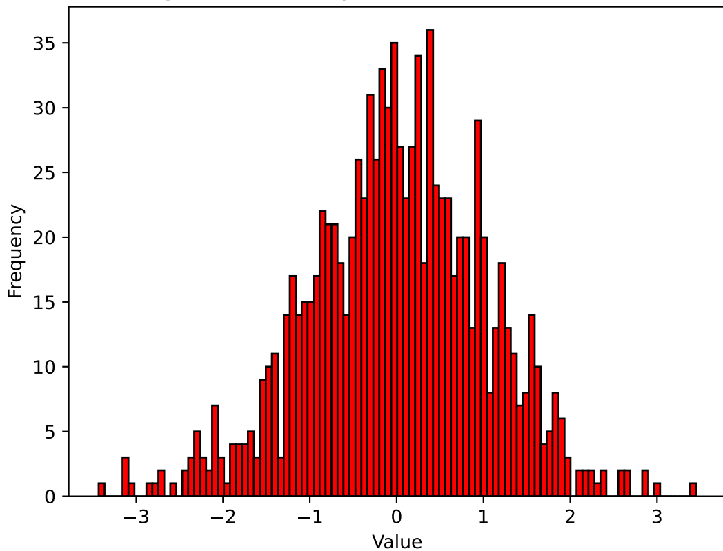
Histogram of Normally Distributed Random Numbers
