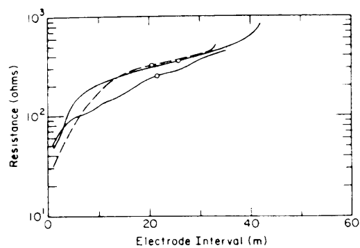
Figure 2-38. Resistance-to-Ground Curves for 3 Electrodes Placed in Holes Modified by Spring Charges and Filled with a Salt-Water Solution.
