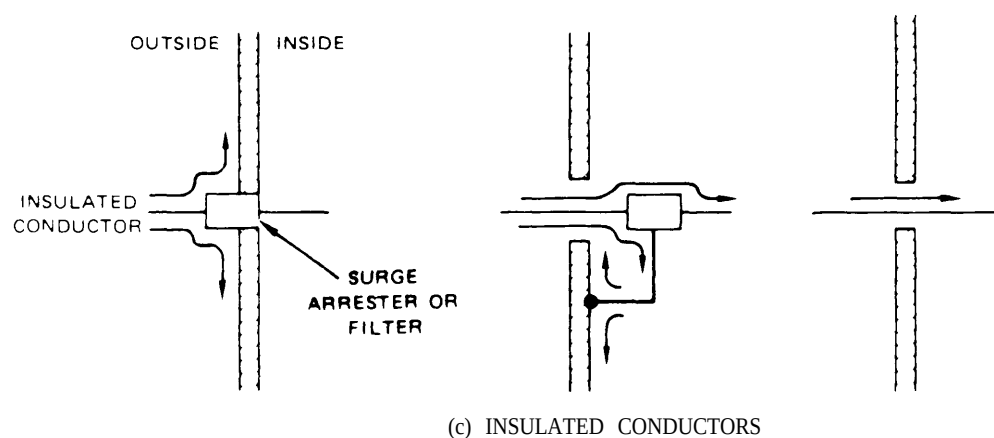
Figure 10-9. Shielding Integrity Near Interference-Carrying External Conductors
