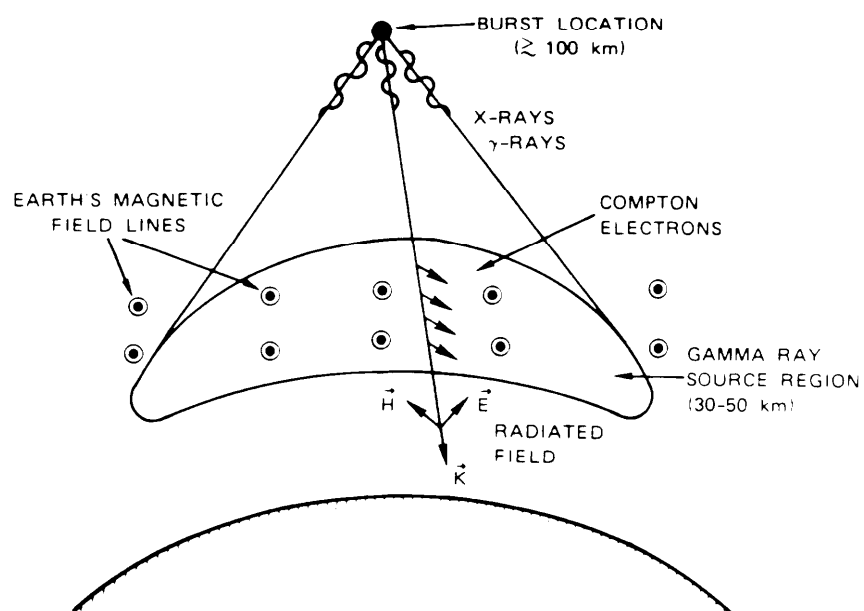
Figure 10-2. Schematic Representation of High-Altitude EMP Generation
