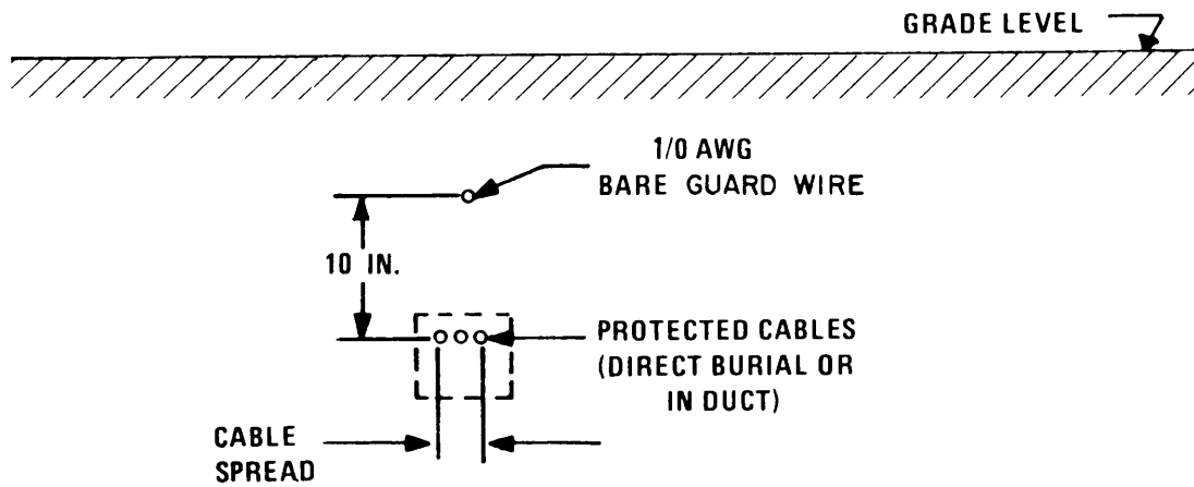
(a) CABLE SPREAD LESS THAN 3 FEET
