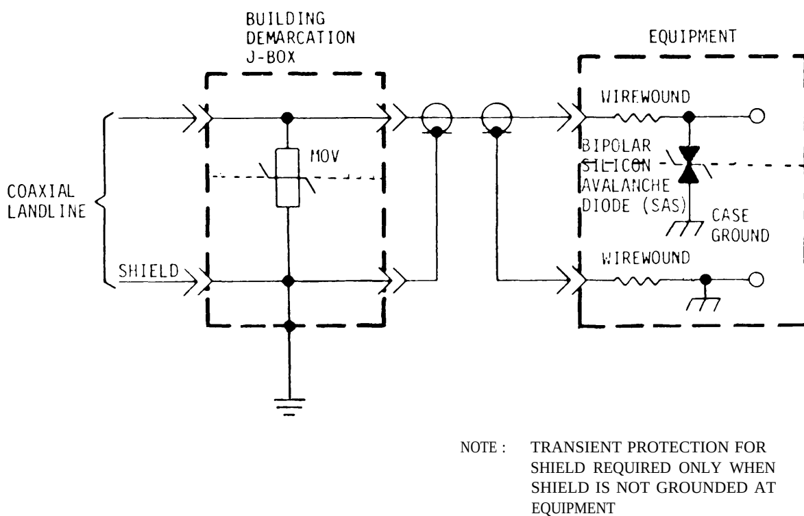
b. TRANSIENT PROTECTION FOR EXTERNALLY-EXPOSED COAXIAL CABLES
