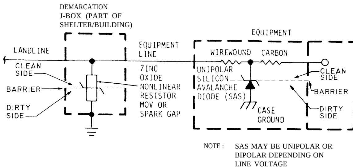
a. TYPICAL TRANSIENT PROTECTION CONFIGURATION
