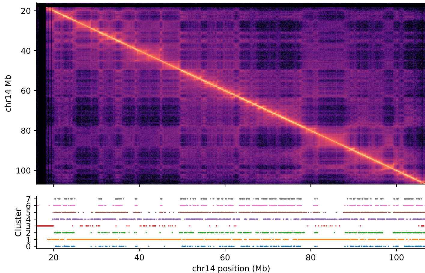
Comprehensive model on GM12878 chr14 Pore-C contact map (100000 bp)
