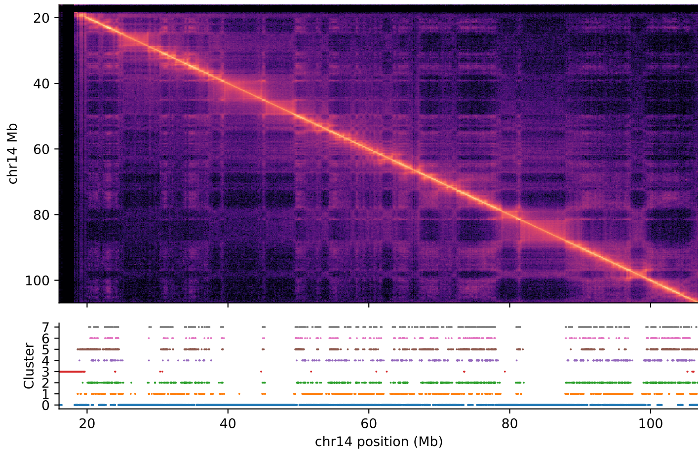
Comprehensive model on K562 chr14 Pore-C contact map (100000 bp)
