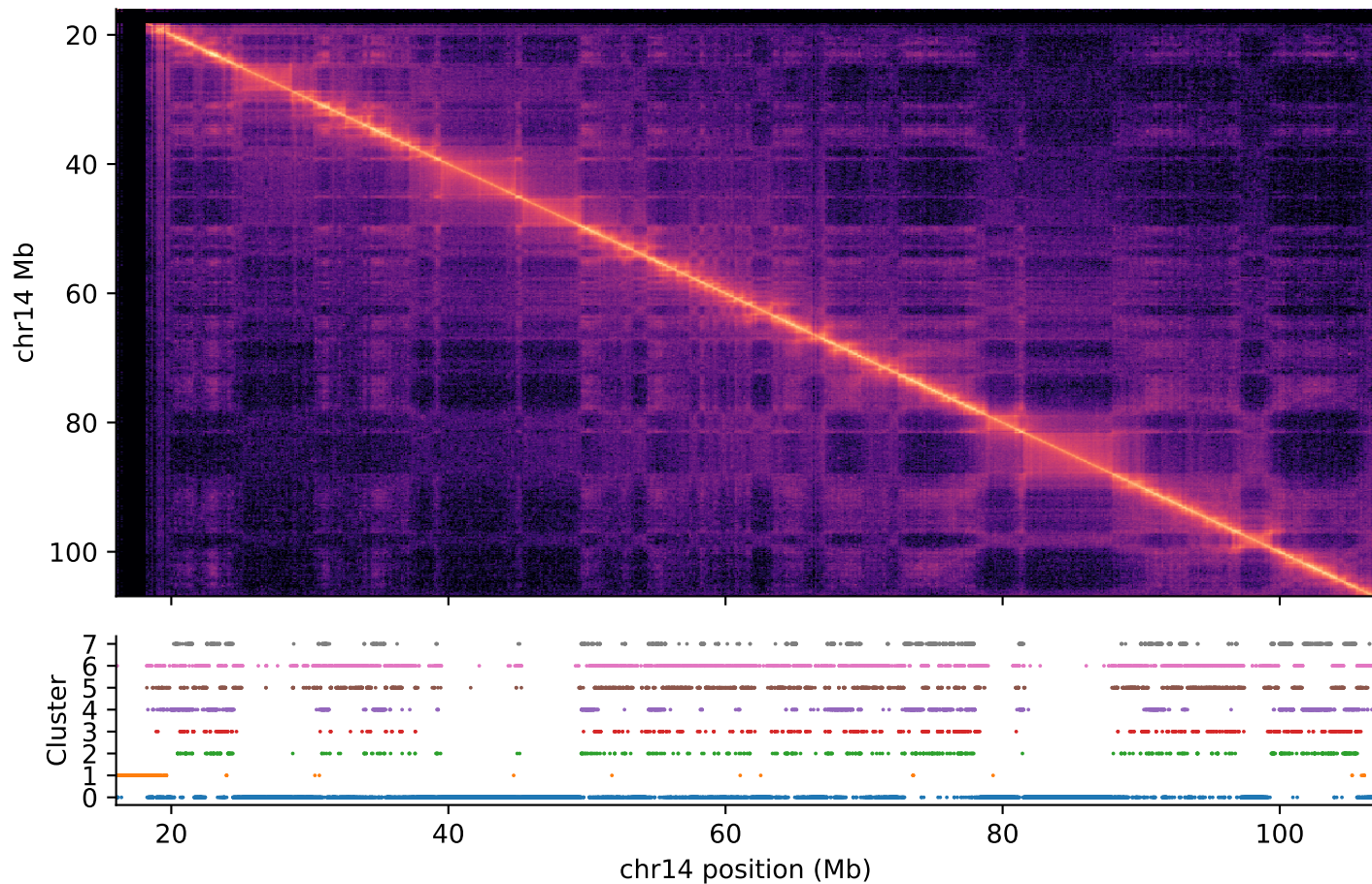
K562 intra-cell model on K562 chr14 Pore-C contact map (100000 bp)
