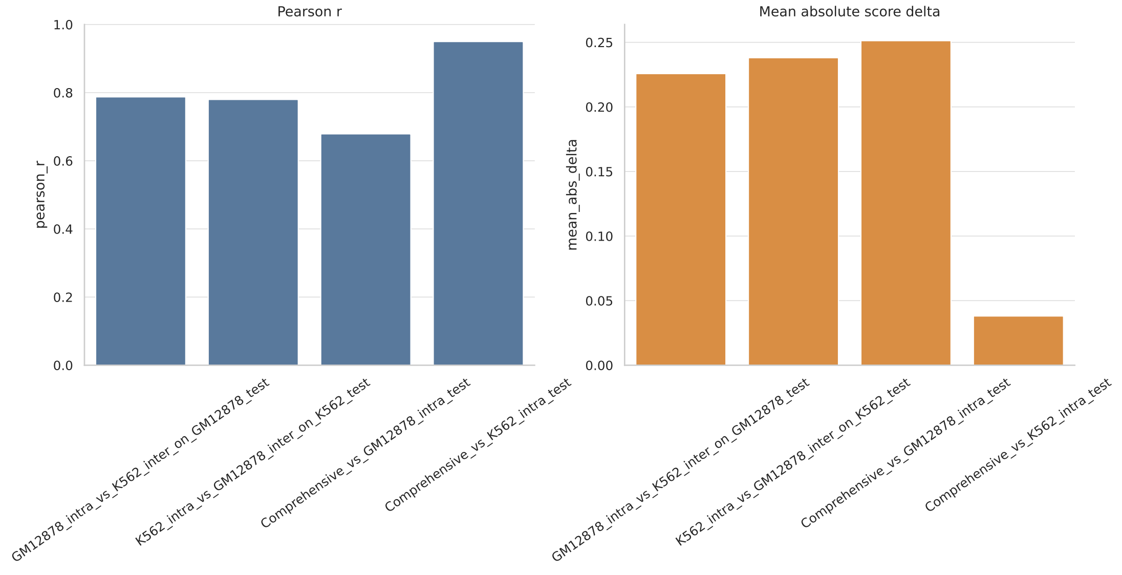
Figure 2k model-score consistency summary
