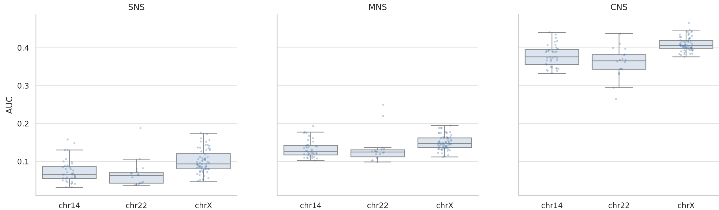
Supplementary Figure 4 inter-cell chromosome AUC
