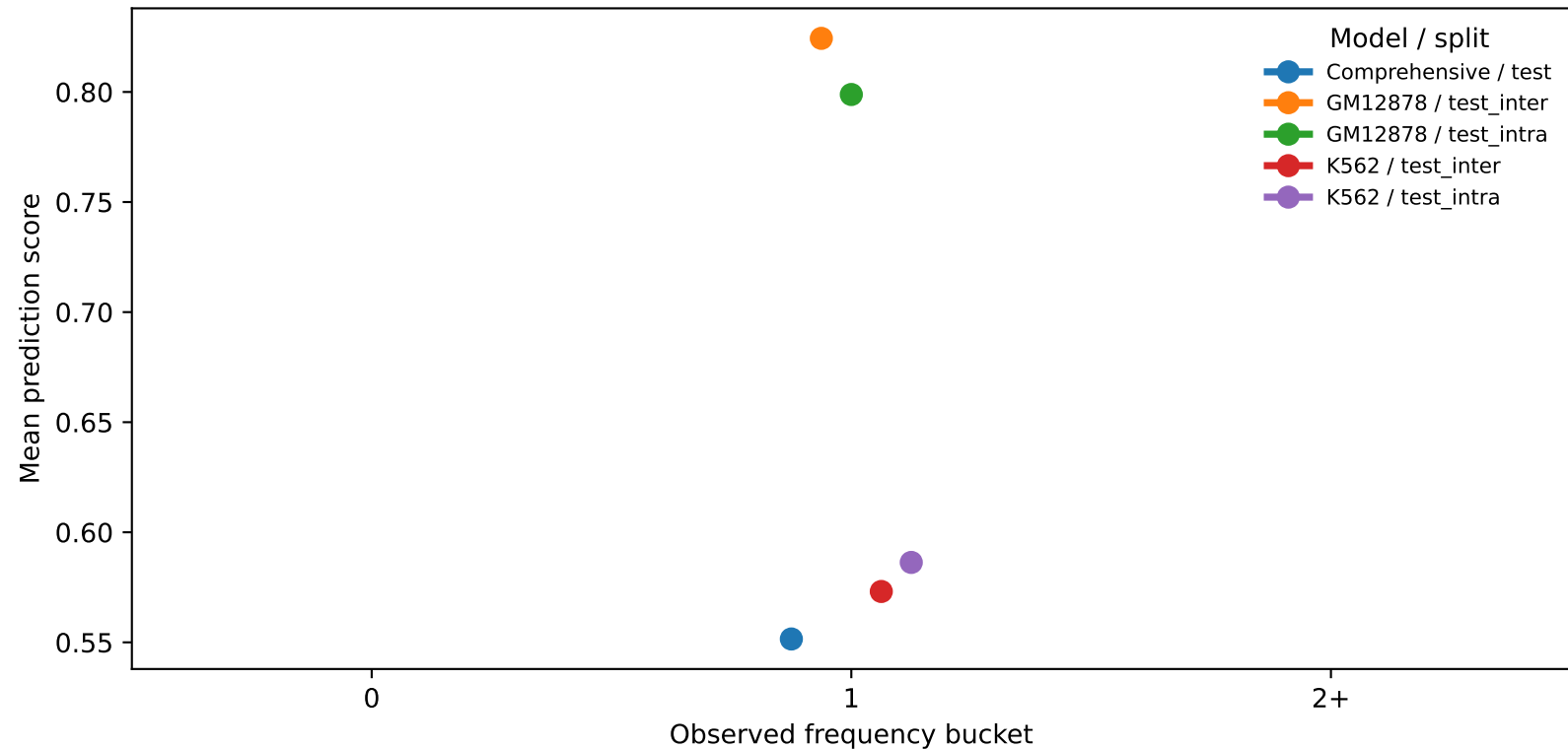
Supplementary Figure 8 observed frequency vs prediction score (maxspan shards: all positives have observed frequency 1)
