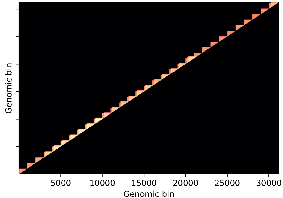
Random choice
