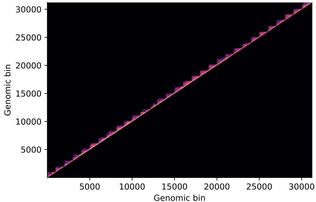
Random walk
