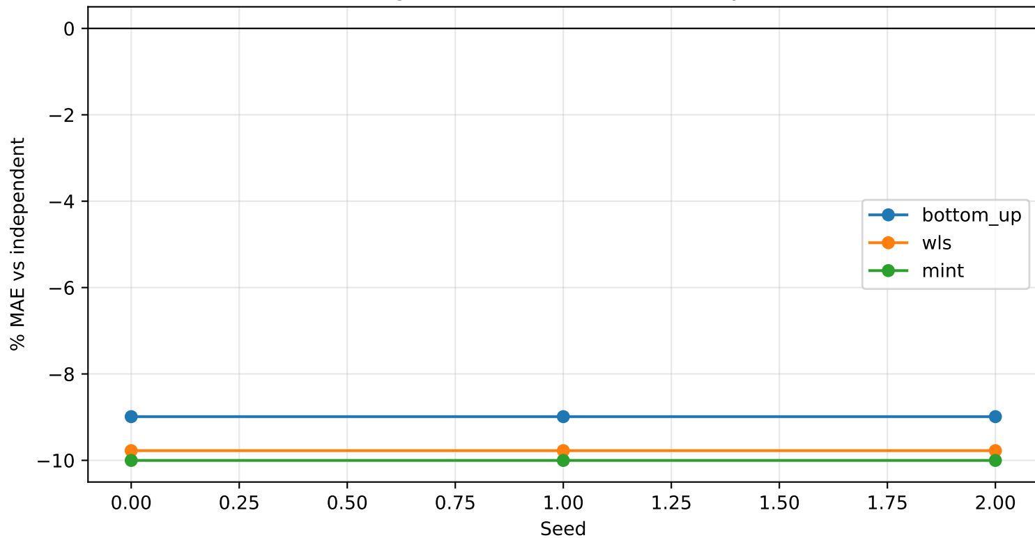
CPU LightGBM reconciliation effect by seed
