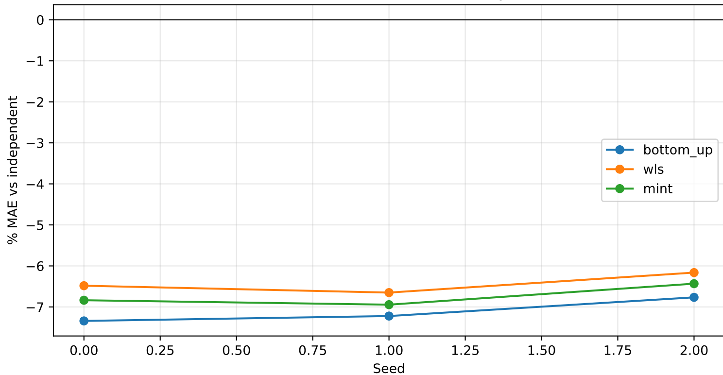
CPU DLinear reconciliation effect by seed
