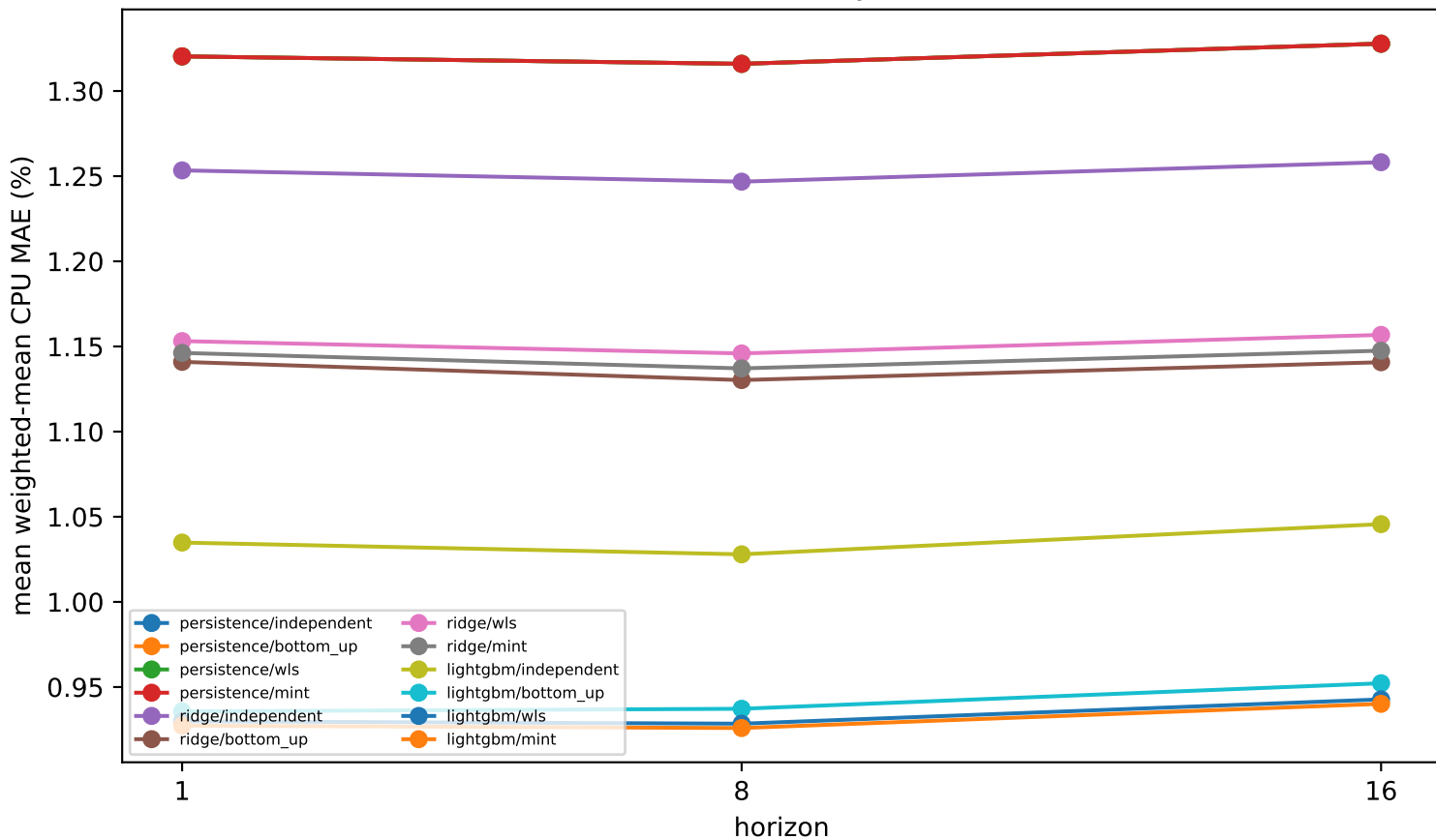
CPU classical accuracy vs horizon
