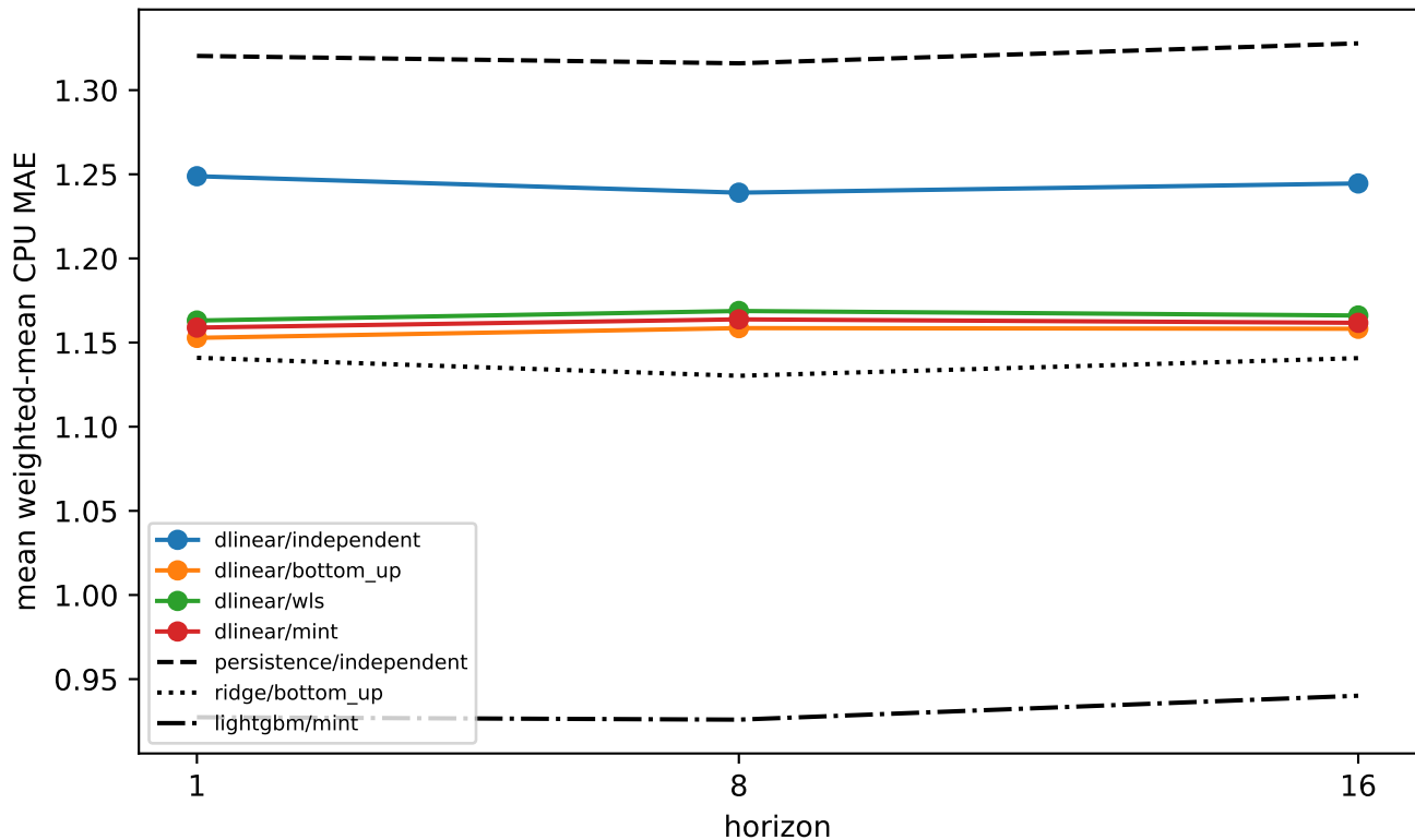
CPU DLinear accuracy vs horizon
