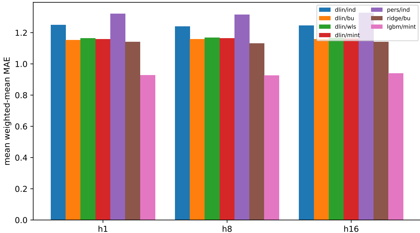
CPU DLinear vs classical
