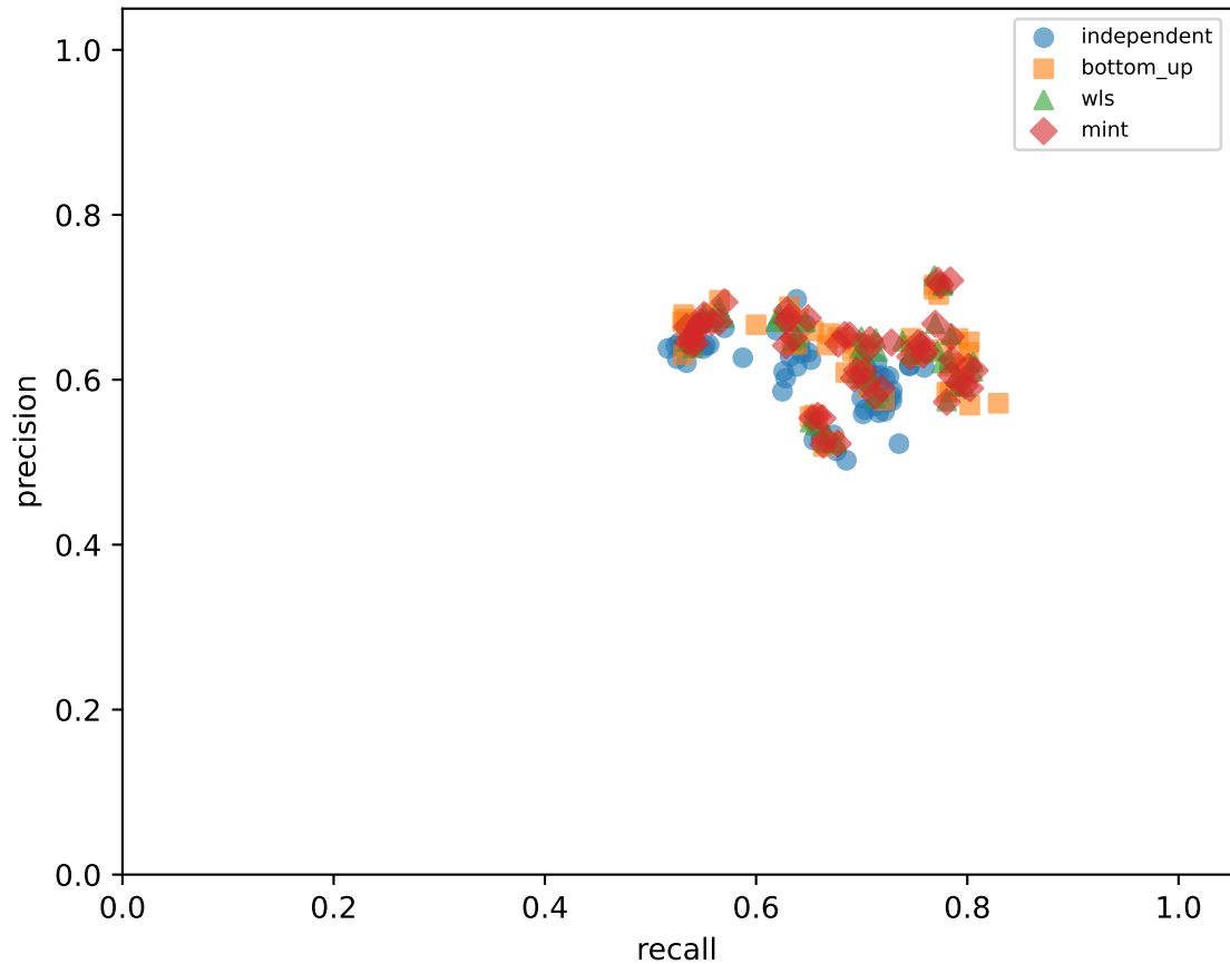
cpu_peak_precision_recall
