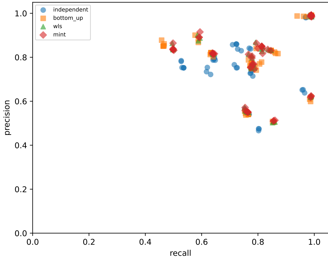
memory_peak_precision_recall
