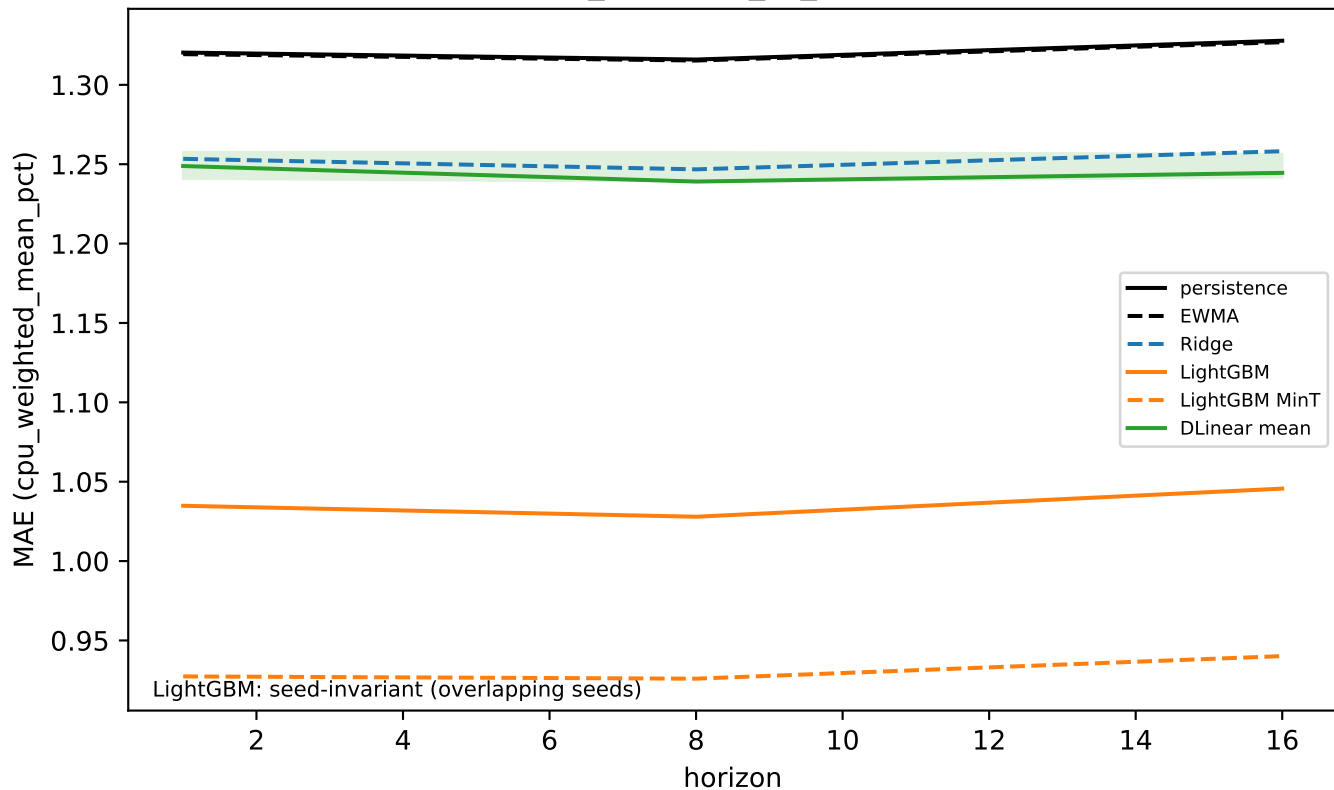
cpu_accuracy_vs_horizon
